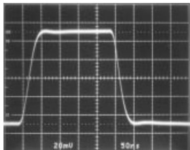
Small-Signal Response
