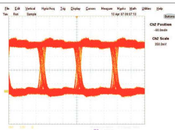
Figure 26. Typical Eye Pattern SN65LVDS179: Tx
