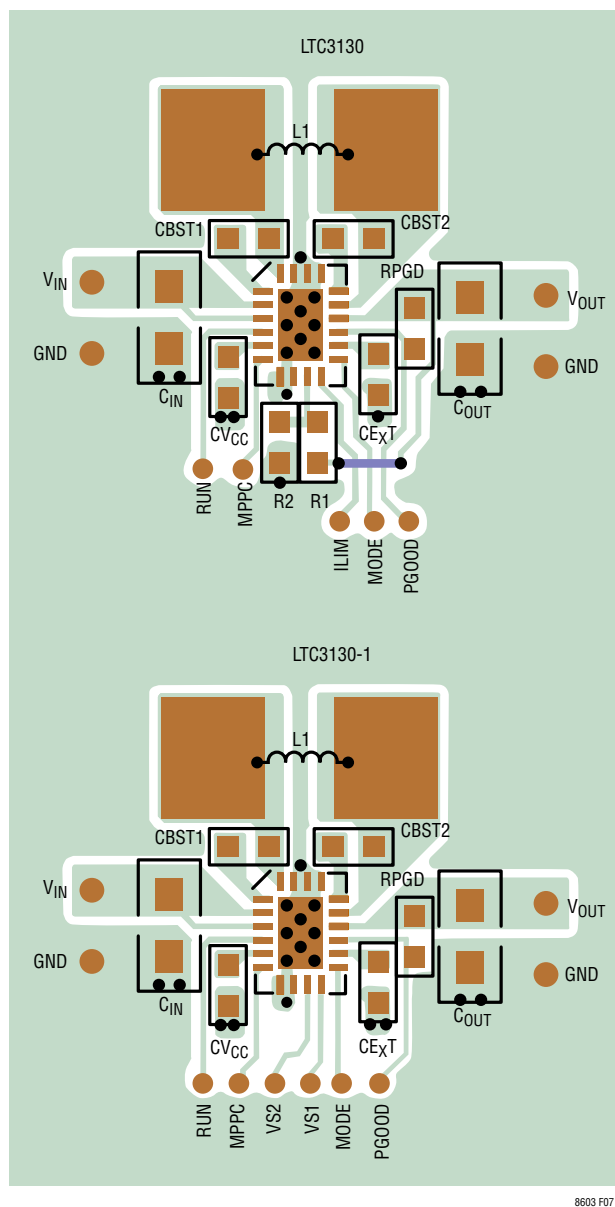
Figure 7. Typical 2-Layer PC Board Layout (QFN Package Shown)
