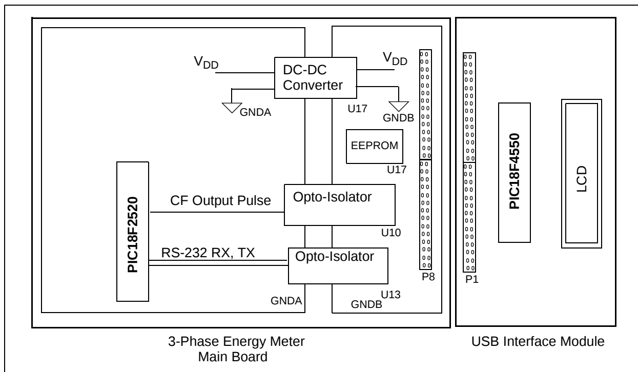
FIGURE 2-3: Meter Output Diagram.
