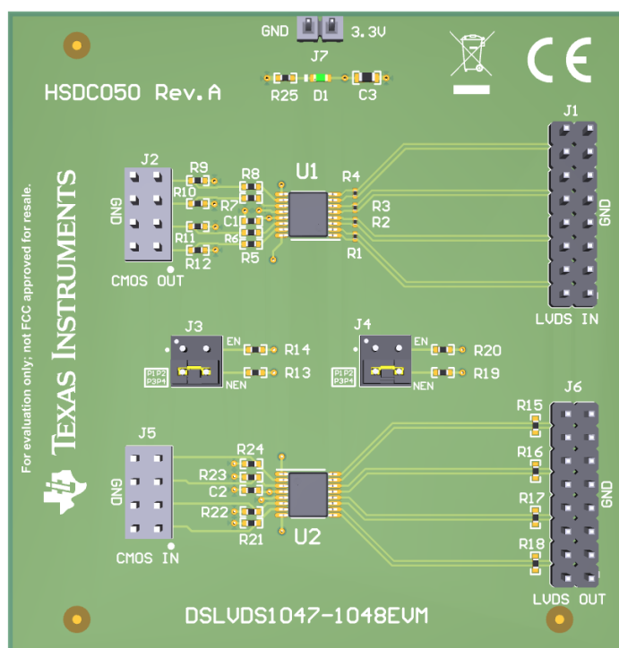
Figure 1. DSLVIDS1047-1048EVM
