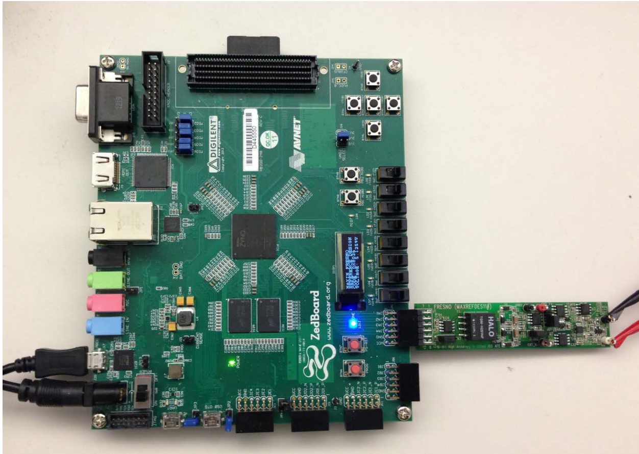
Figure 1. Fresno Board Connected to ZedBoard Kit
