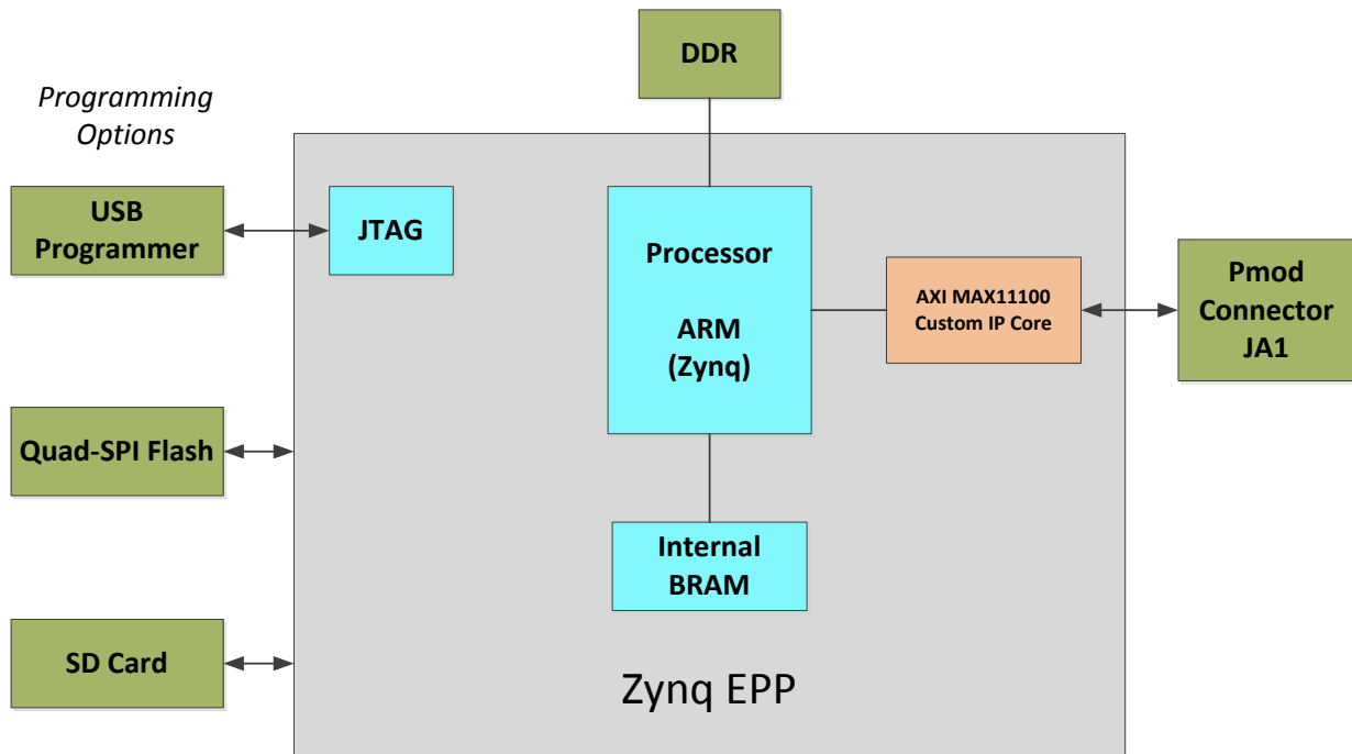
Figure 3. Block Diagram of FPGA Hardware Design
