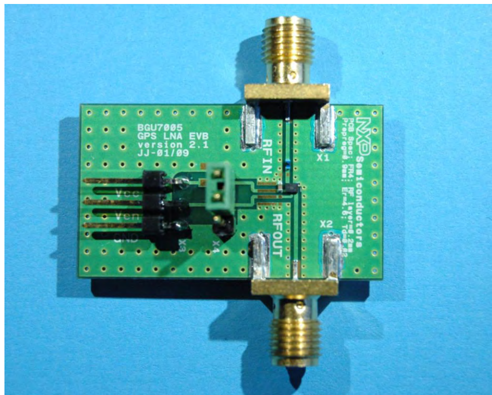
Fig 1. BGU7004 GPS LNA evaluation board
