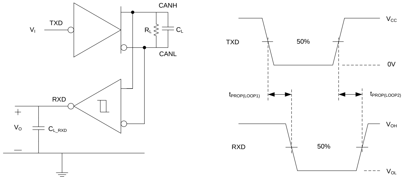
Figure 10. t_{\text{PROP(LOOP)}} Test Circuit and Measurement
