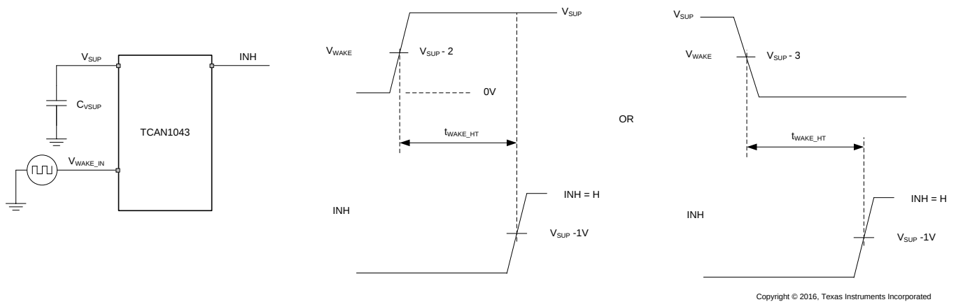
Figure 16. t_{\text{Wake\_HT}} While Monitoring INH Output
