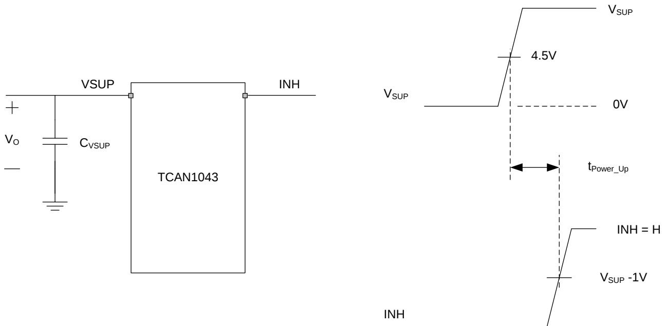
Figure 15. t_{\text{Power\_Up}} Timing Measurement
