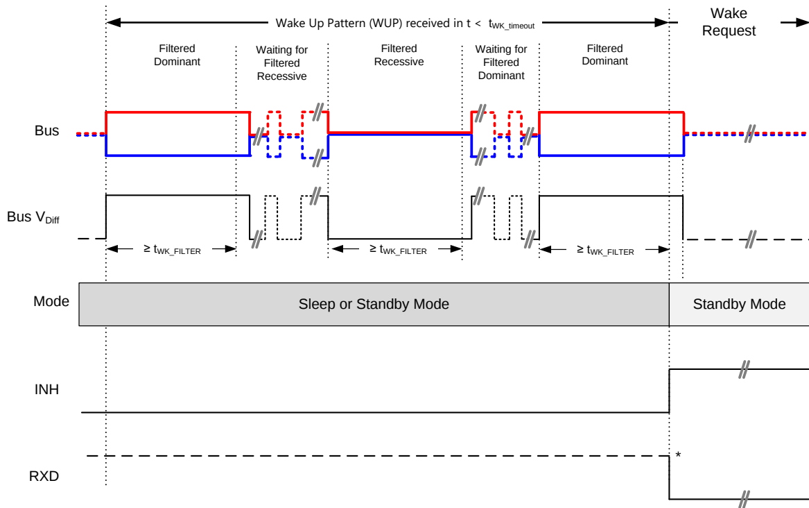
Figure 22. Wake Up Pattern (WUP)
