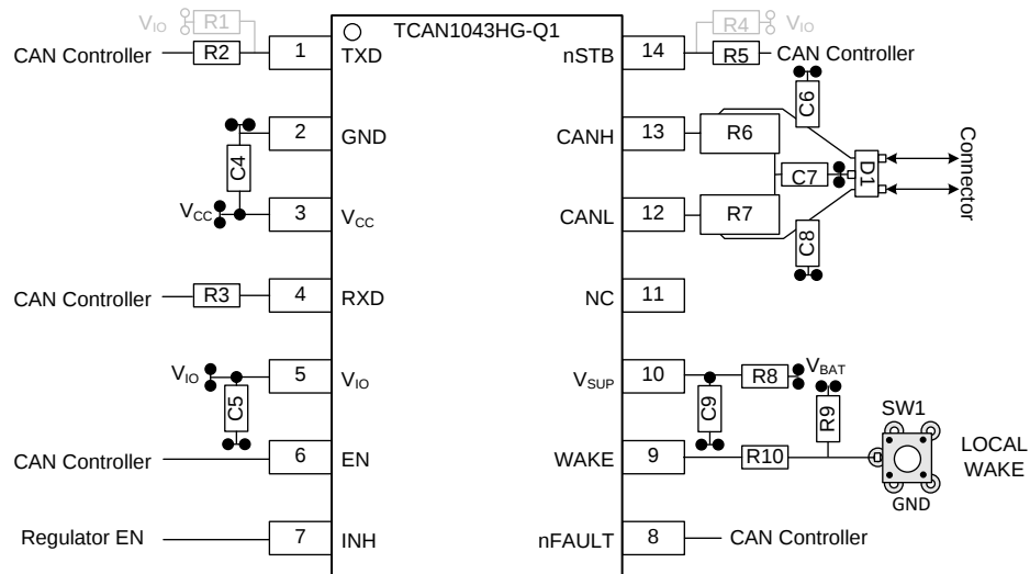
Figure 31. TCAN1043xx-Q1 Layout Example
