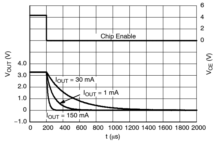
Figure 37. Shutdown, 3.3 V Version D, V_{IN} = 4.3 \text{ V}
