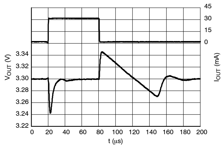
Figure 29. Load Transients, 3.3 V Version, I_{OUT} = 1 - 30 mA, t_R = t_F = 0.5 \mu s, V_{IN} = 4.3 V
