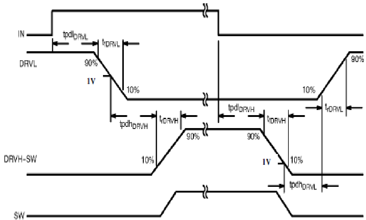
Figure 3. Timing Diagram
