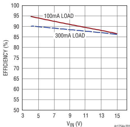
Figure 1. DC1754A Efficiency in PWM Mode
