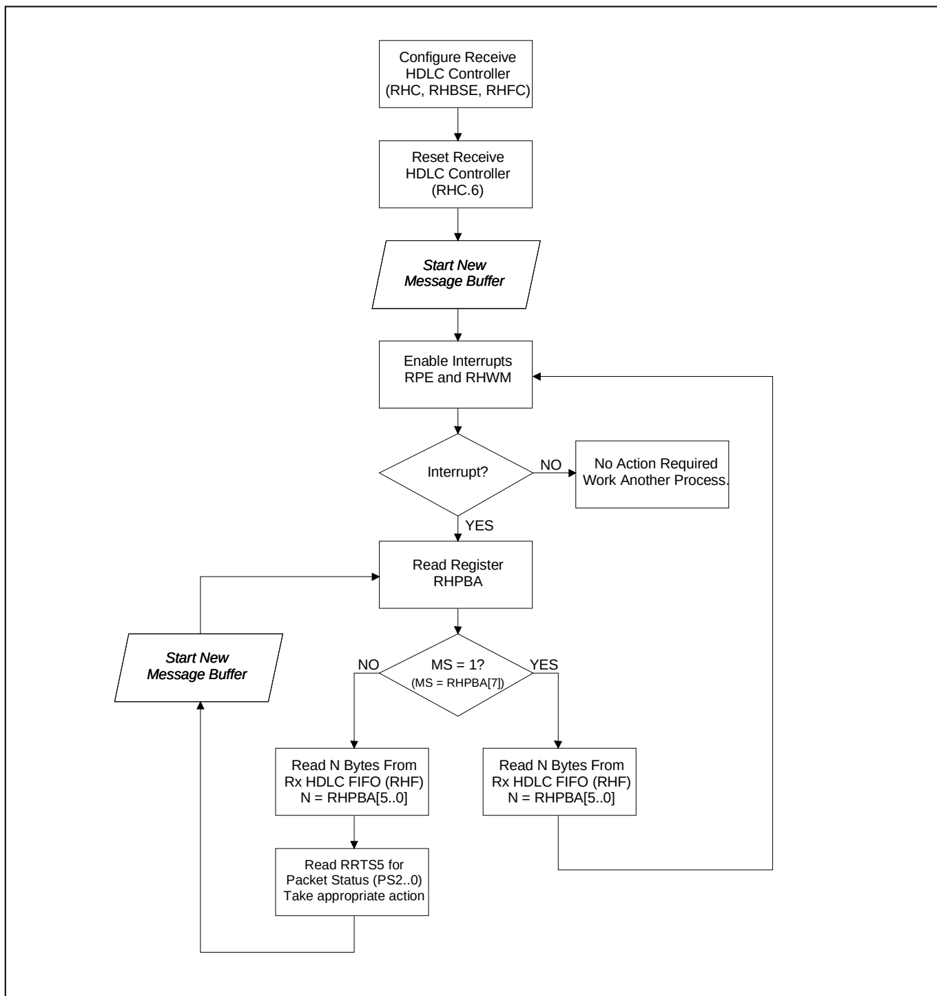
Figure 9-17. HDLC Message Receive Example
