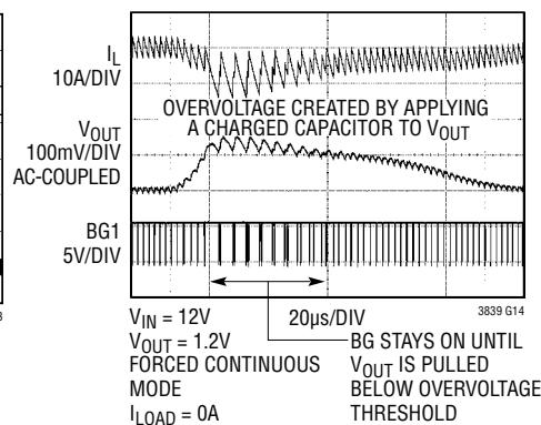
Overvoltage Protection
