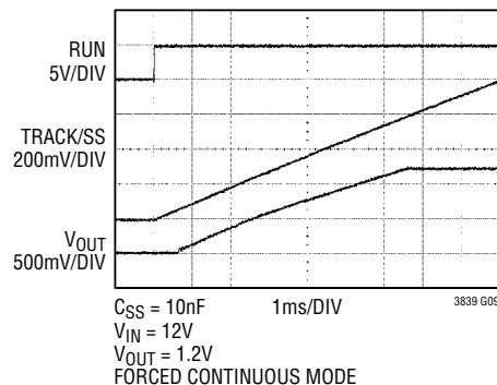
Regular Soft Start-Up
