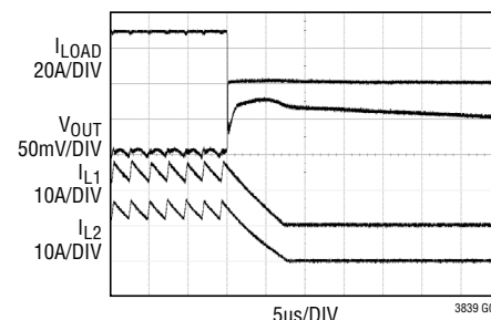
Load Release (Discontinuous Mode)
