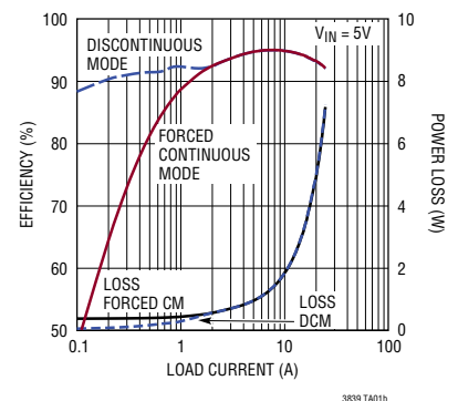
Efficiency/Power Loss
