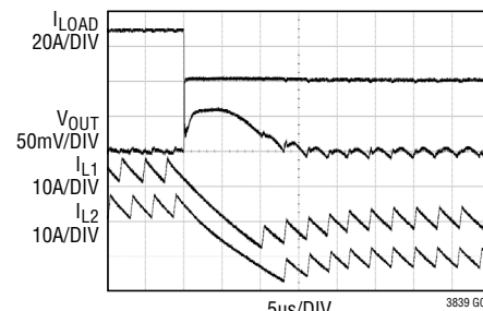
Load Release (Forced Continuous Mode)
