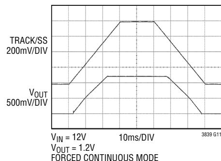
Output Tracking
