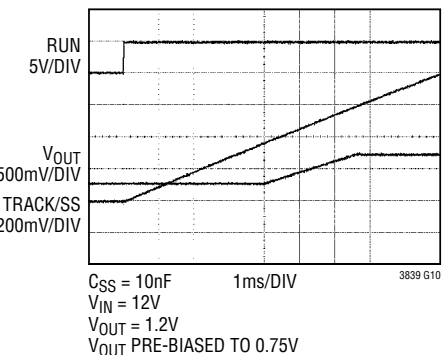
Soft Start-Up Into Pre-Biased Output
