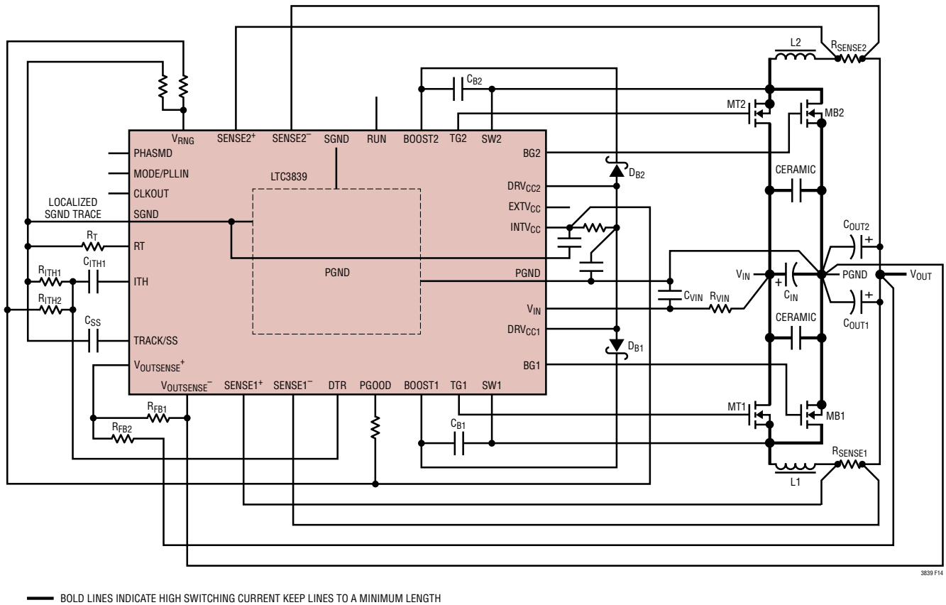
Figure 14. Recommended PCB Layout Diagram
