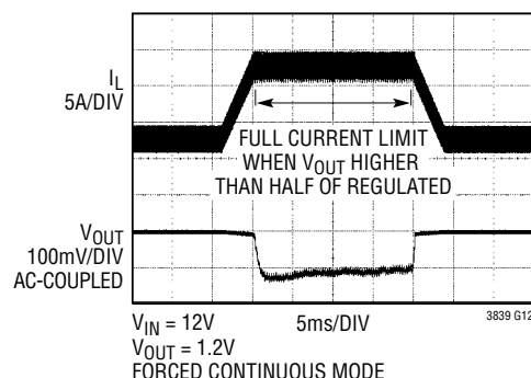
Overcurrent Protection
