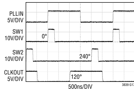
Phase Relationship: PHASMD = INTV CC
