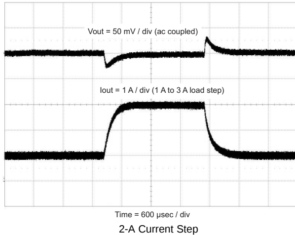
Figure 40. Transient Response
