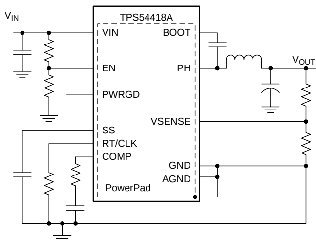
Simplified Schematic
