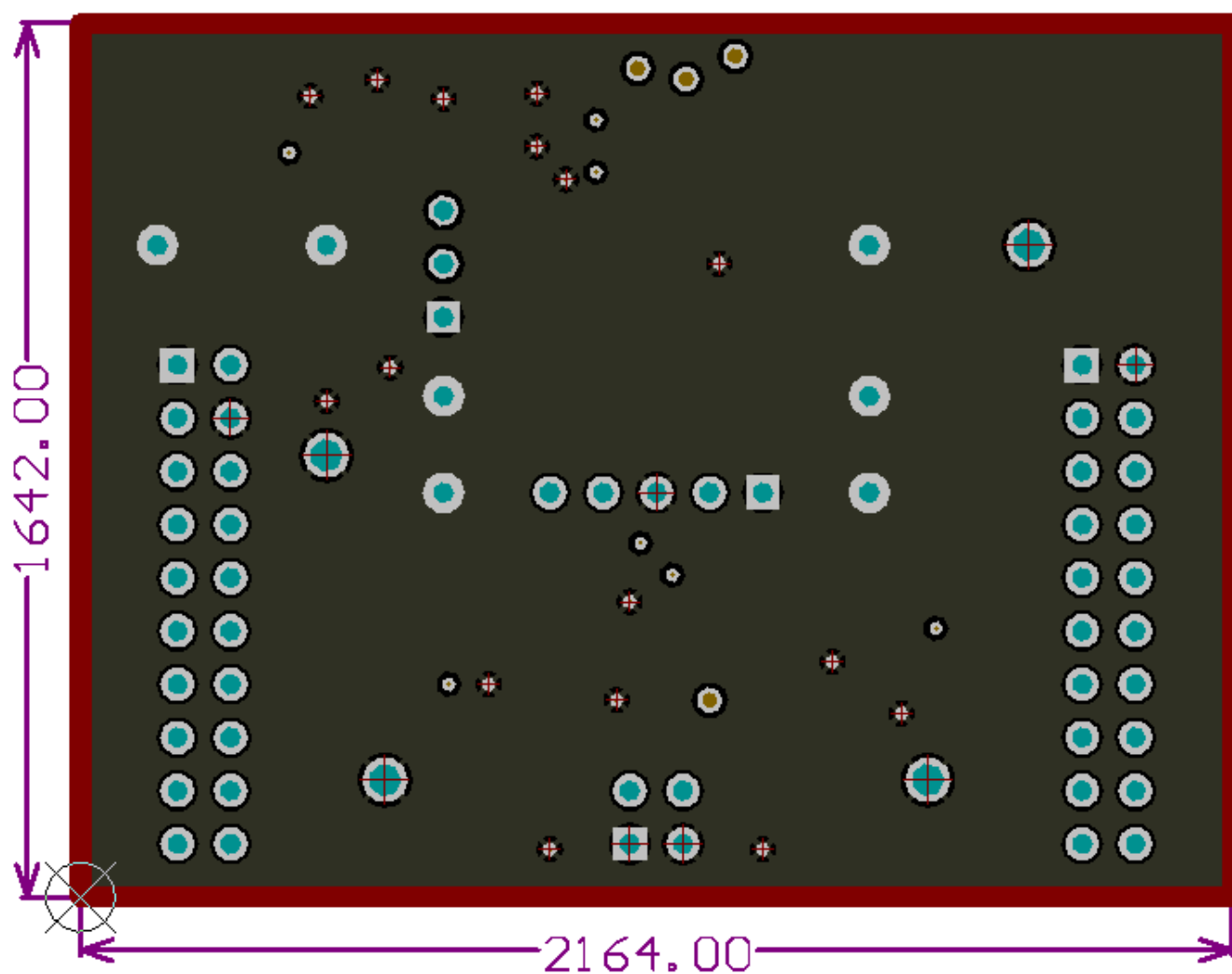
Figure 20. Ground Layer Routing
