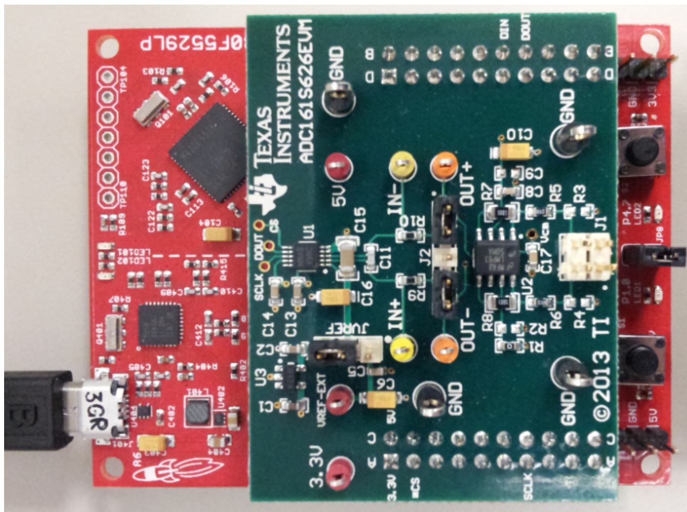
Figure 13. ADC161S626EVM Hardware Connection
