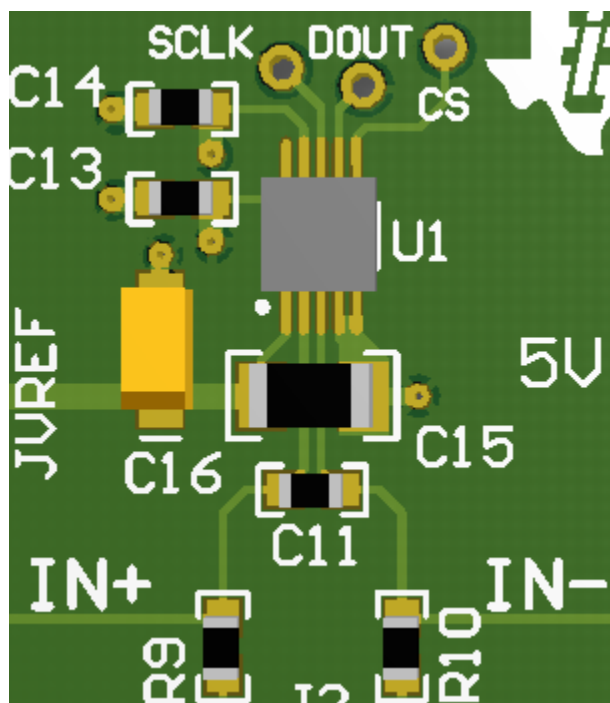
Figure 6. The ADC161S626 Circuit
