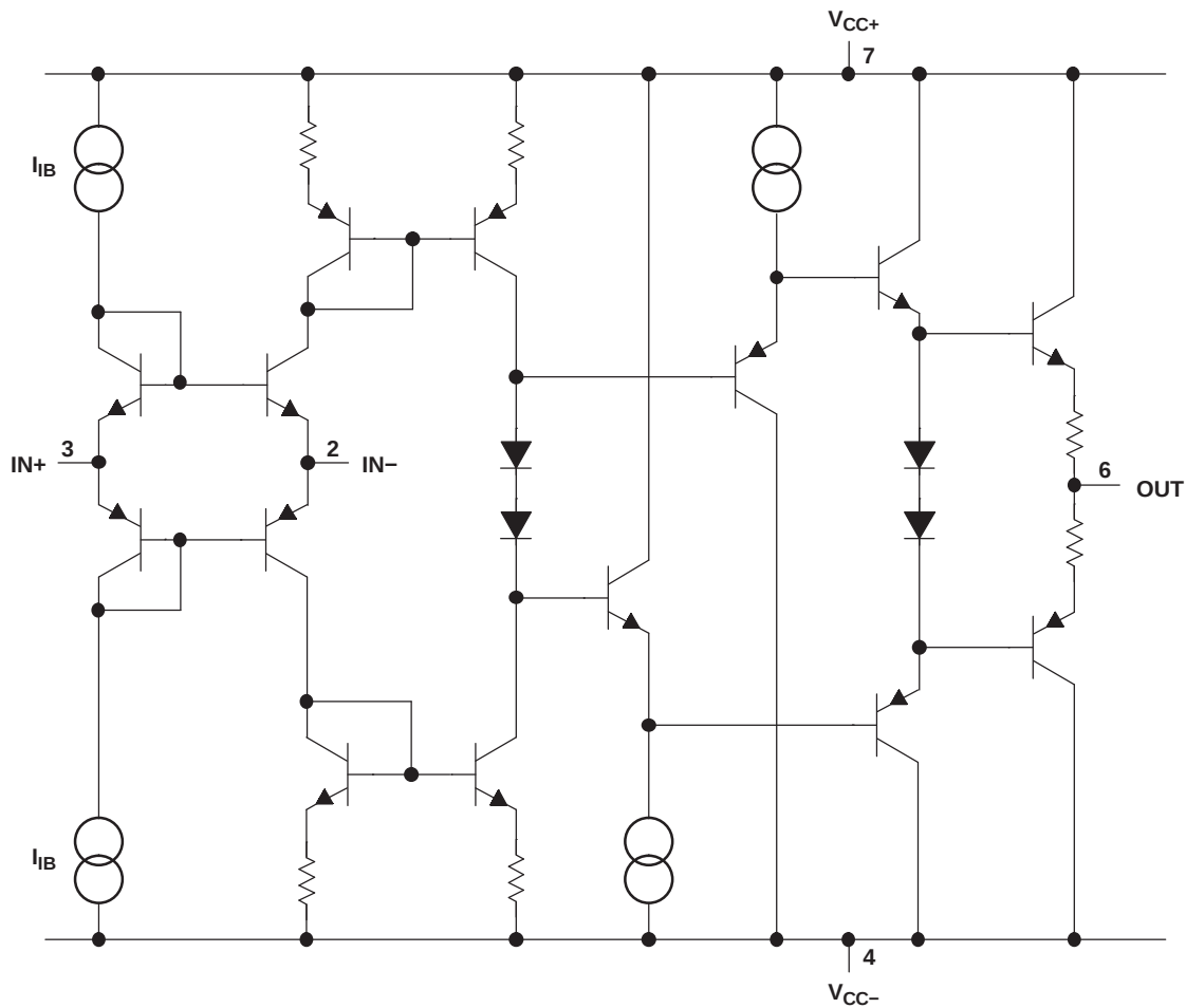
Figure 47. Simplified Schematic
