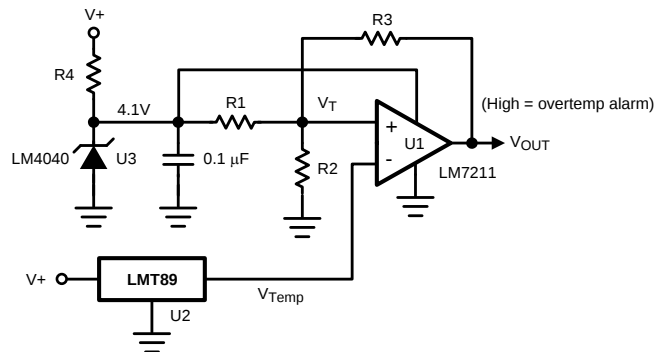
Figure 6. Centigrade Thermostat
