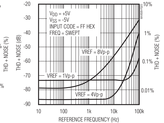
REFERENCE VOLTAGE INPUT FREQUENCY RESPONSE
