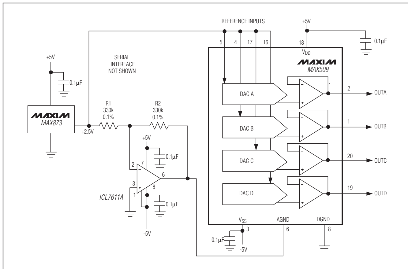
Figure 14. MAX509 AGND Bias Circuit (Negative Offset)
