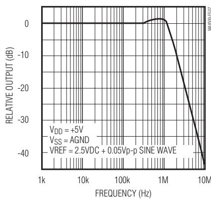
REFERENCE VOLTAGE INPUT FREQUENCY RESPONSE
