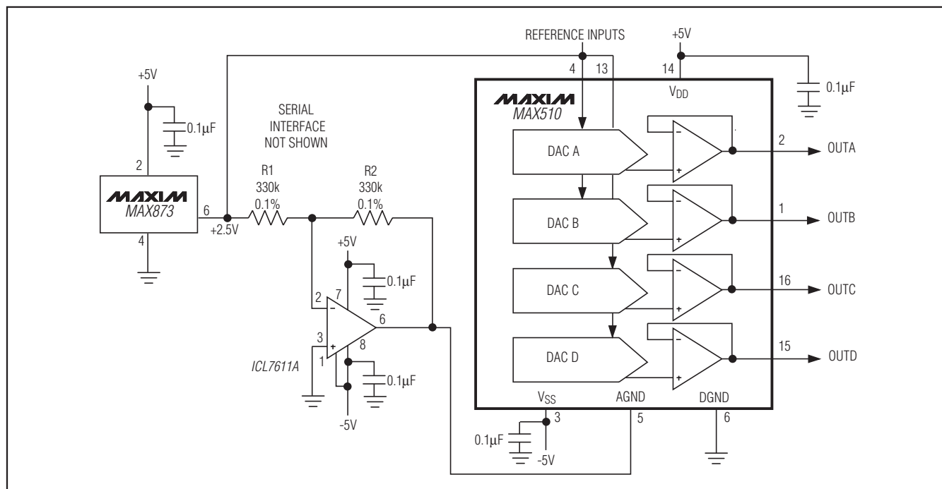
Figure 15. MAX510 AGND Bias Circuit (Negative Offset)
