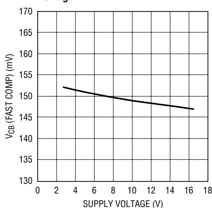
V_{CB} (FAST COMP) vs Supply Voltage
