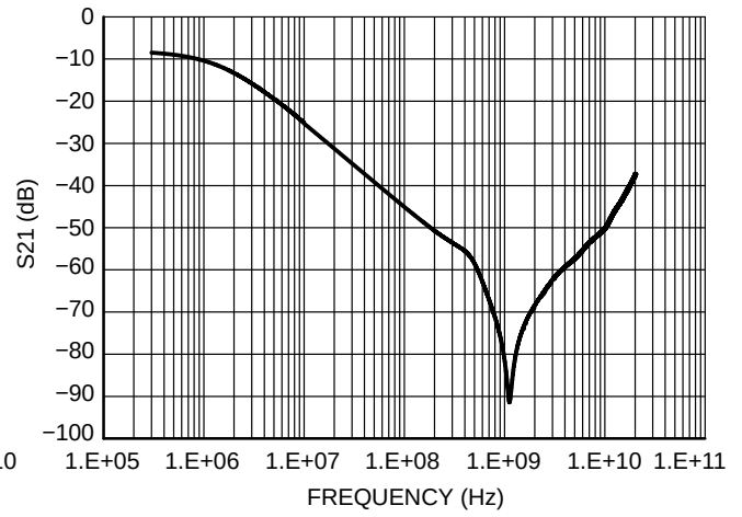
Figure 3. Typical Insertion Loss (450 \Omega Source and 10 k \Omega Load Termination)
