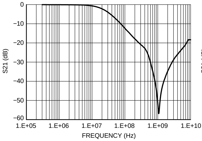
Figure 1. Typical Insertion Loss (50 \Omega Termination)
