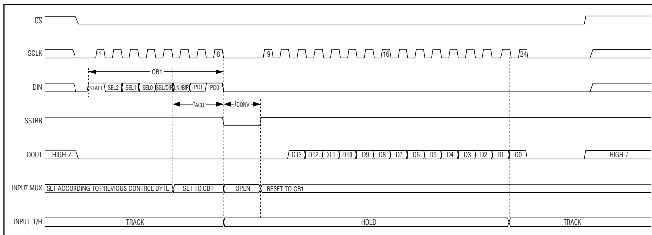
Figure 9. Internal Clock Mode Timing—24 Clocks/Conversion Timing
