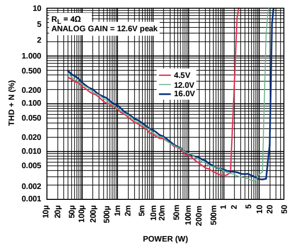
Figure 23. THD + N vs. Power, R_L = 4\Omega , Analog Gain = 12.6 V peak
