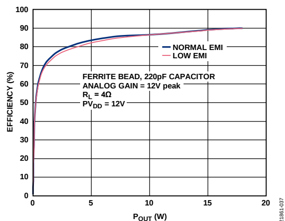
Figure 39. Efficiency vs. P_{OUT} with Ferrite Bead, Analog Gain = 12 V peak, R_L = 4\ \Omega , PV_{DD} = 12\text{ V}
