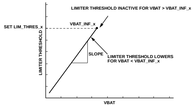
Figure 83. Limiter Threshold vs. VBAT in Limiter Tracking Mode (LIM_EN_x = 11, VBAT_TRACK_x = 1)
