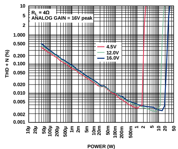
Figure 24. THD + N vs. Power, R_L = 4\Omega , Analog Gain = 16 V peak
