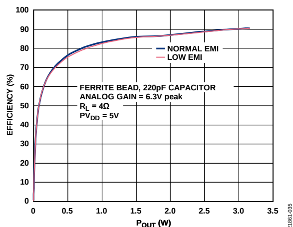
Figure 37. Efficiency vs. P_{OUT} with Ferrite Bead, Analog Gain = 6.3 V peak, R_L = 4\ \Omega , PV_{DD} = 5\text{ V}
