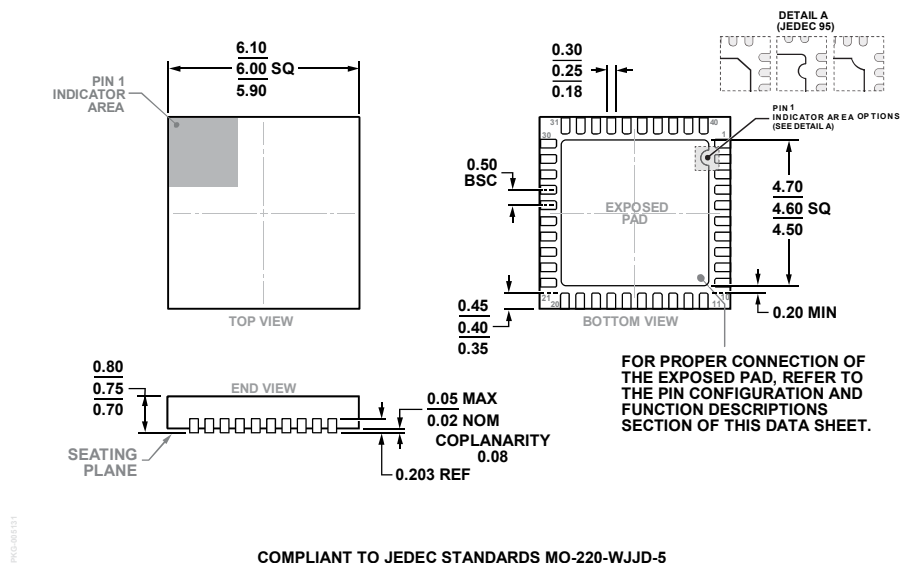
Figure 88. 40-Lead Lead Frame Chip Scale Package [LFCSP] 6 mm × 6 mm Body and 0.75 mm Package Height (CP-40-7)
