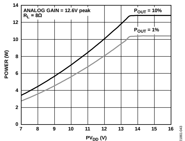
Figure 45. Power vs. PV DD , Analog Gain = 12.6 V peak, R_L = 8\Omega
