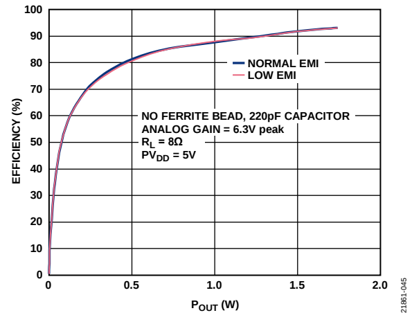
Figure 47. Efficiency vs. P OUT , No Ferrite Bead, Analog Gain = 6.3 V peak, R_L = 8\Omega , PV DD = 5 V
