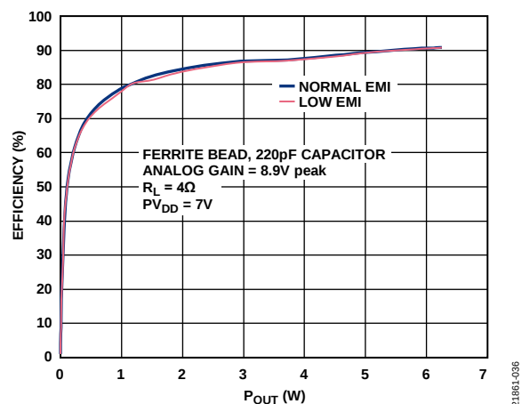
Figure 38. Efficiency vs. P_{OUT} with Ferrite Bead, Analog Gain = 8.9 V peak, R_L = 4\ \Omega , PV_{DD} = 7\text{ V}
