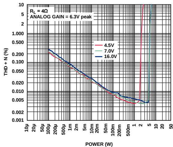
Figure 21. THD + N vs. Power, R_L = 4\Omega , Analog Gain = 6.3 V peak
