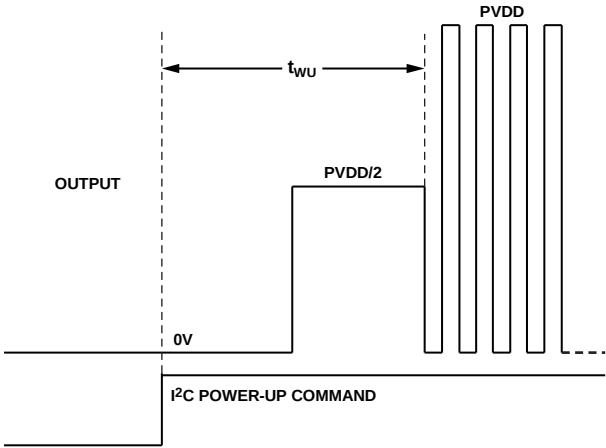
Figure 4. Turn On Time, Hard Volume
