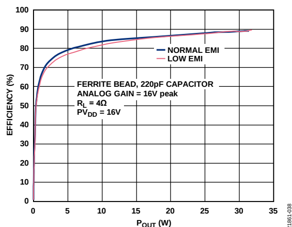
Figure 40. Efficiency vs. P_{OUT} with Ferrite Bead, Analog Gain = 16 V peak, R_L = 4\ \Omega , PV_{DD} = 16\text{ V}
