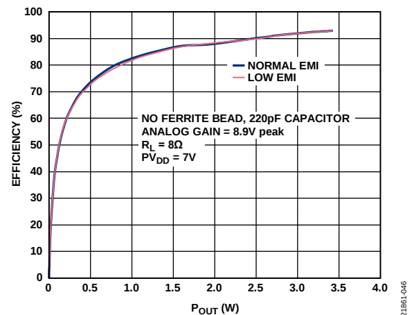
Figure 48. Efficiency vs. P OUT , No Ferrite Bead, Analog Gain = 8.9 V peak, R_L = 8\Omega , PV DD = 7 V
