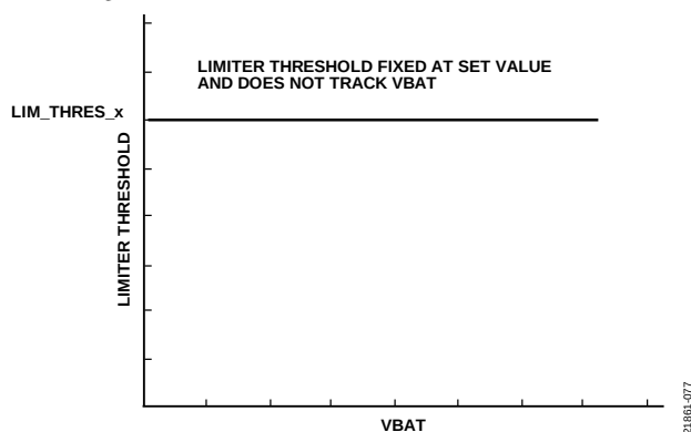
Figure 76. Limiter Fixed (LIM_EN_x = 0b01, VBAT_TRACK_x = 0b0)
