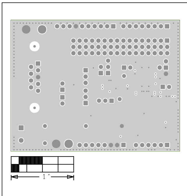
MAX33053E Shield—Internal 2
