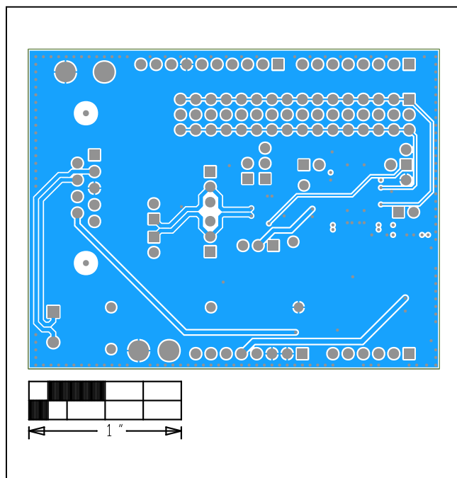
MAX33053E Shield—Bottom
