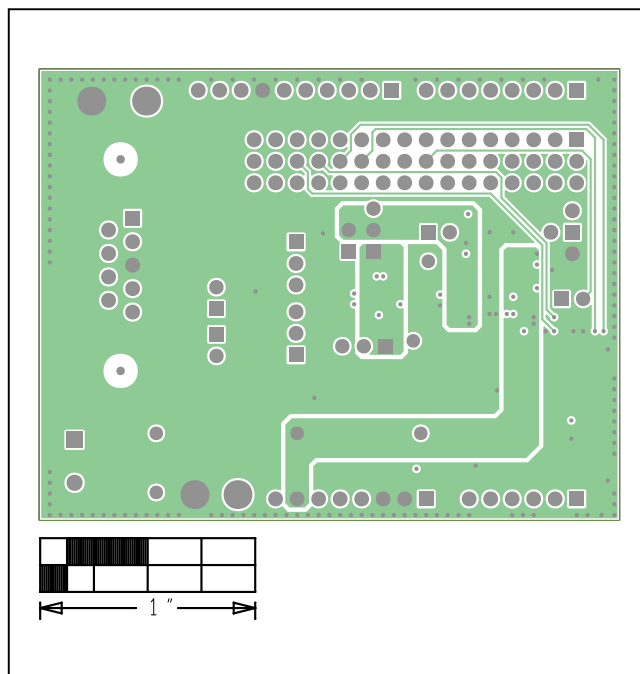
MAX33053E Shield—Internal 3
