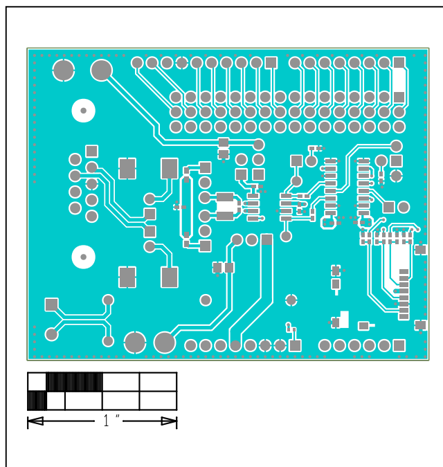
MAX33053E Shield—Top
