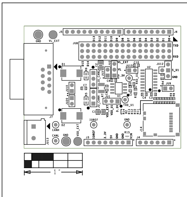
MAX33053E Shield—Top Silkscreen
