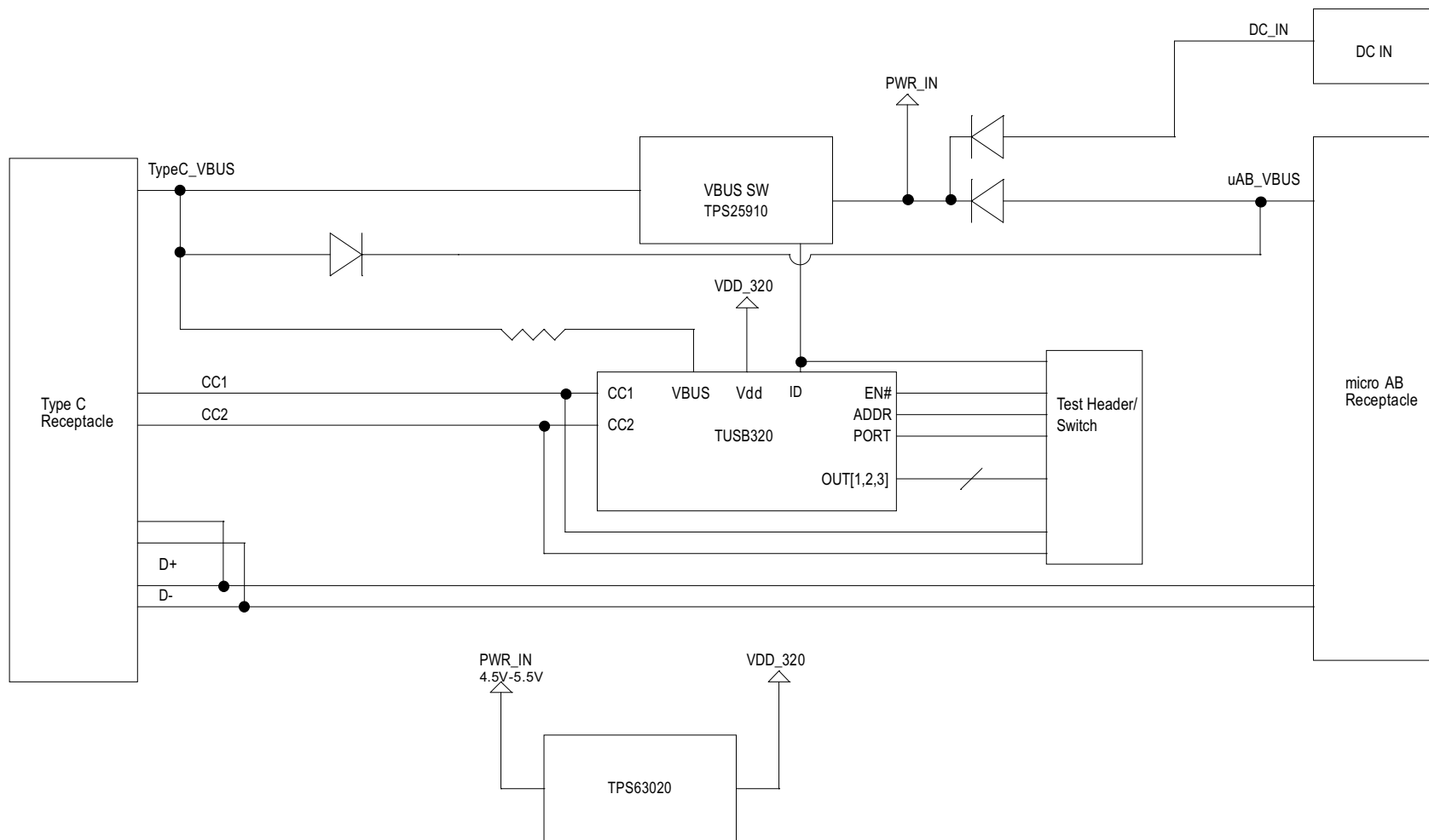
Figure 5. TUSB320 EVM Schematic
