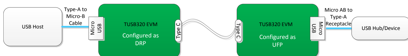
Figure 3. Example Configuration Using HD3SS2522 and TUSB320 EVMs
