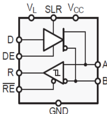
Figure 4. Block diagram
