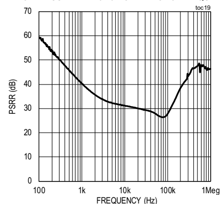
MAX17671F, 3.3V LINEAR REGULATOR POWER SUPPLY REJECTION RATIO vs. FREQUENCY
