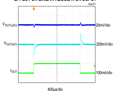
MAX17671F, 3.3V LINEAR REGULATOR LOAD TRANSIENT ON STEP-DOWN CONVERTER AND ITS EFFECT ON LINEAR REGULATOR OUTPUT
