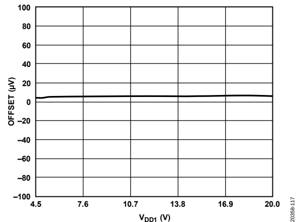
Figure 17. Offset vs. V_{DD1}
