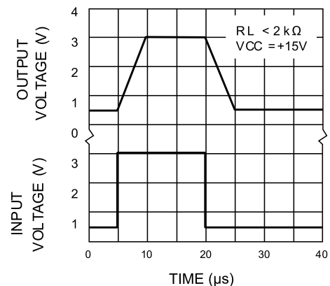
Figure 8: Voltage follower pulse response ( V_{CC} = 15 V )
