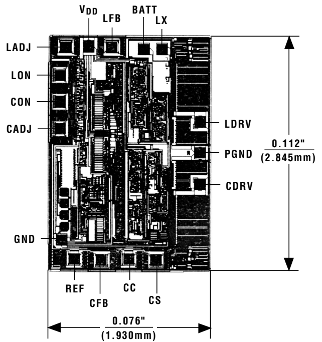
Chip Topography
