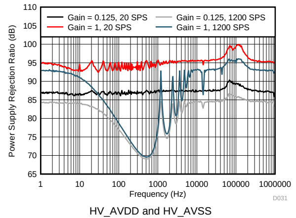
Figure 49. PSRR vs Frequency
