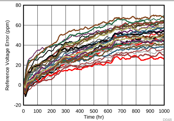
Figure 39. Internal Reference Voltage Drift Distribution
