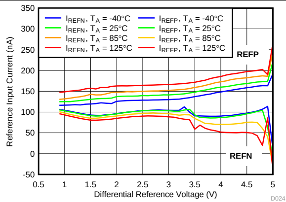
Figure 42. Reference Input Current vs Reference Voltage
