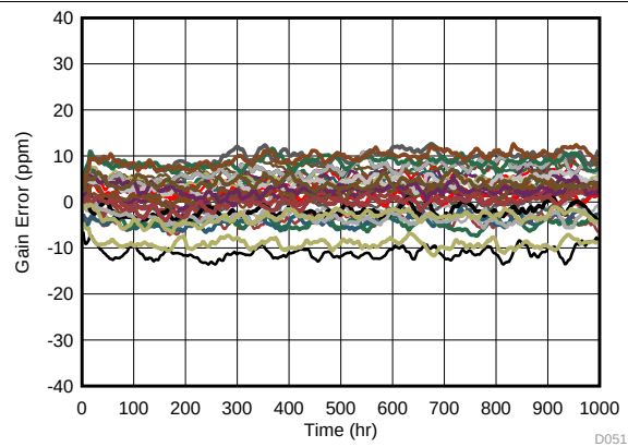
Figure 36. Gain Long-Term Drift
