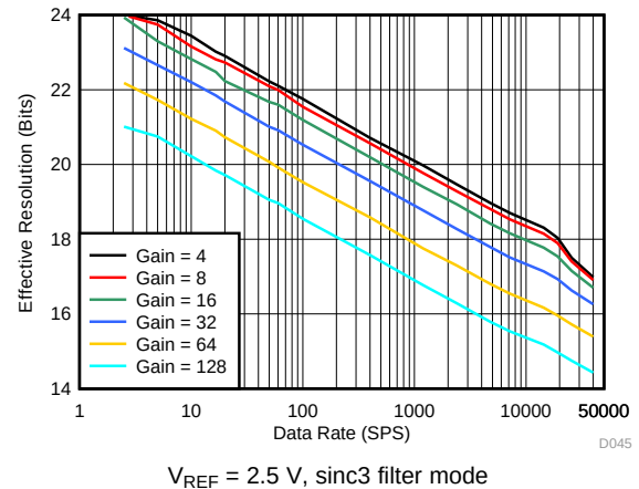
Figure 53. Effective Resolution, Gain = 4 to 128
