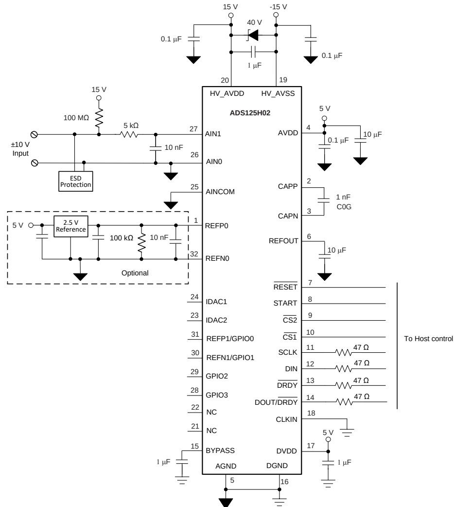
Figure 98. \pm 10 -V Analog Input PLC Module
