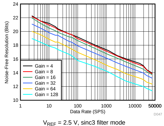
Figure 55. Noise-Free Resolution, Gain = 4 to 128
