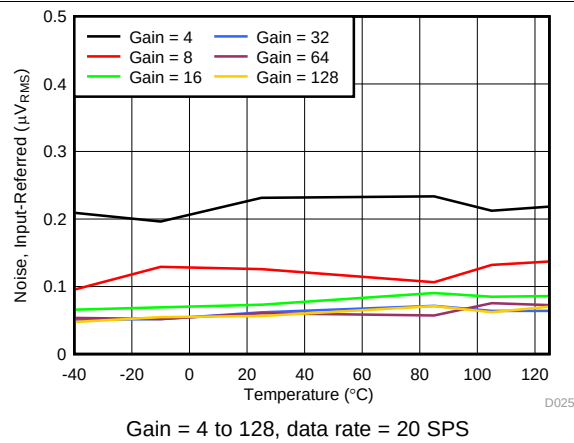
Figure 12. Noise vs Temperature
