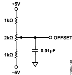
Figure 20. Circuit to Control V_{\text{OFFSET}} ( \pm 2.5 V)
