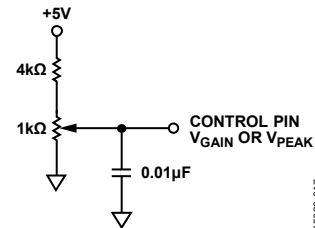
Figure 19. Circuit to Control V_{\text{GAIN}} and V_{\text{PEAK}} (0 V to 1 V)
