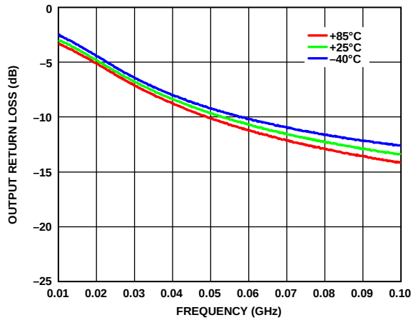
Figure 32. Output Return Loss vs. Frequency (10 MHz to 100 MHz), State = Internal Amplifier (Refer to Figure 76 for the Test Circuit)
