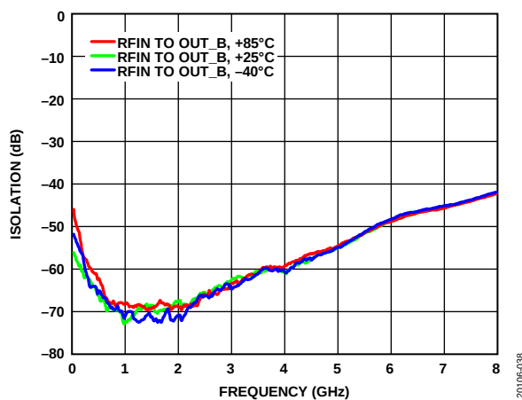
Figure 34. Isolation vs. Frequency Over Temperature, State = Internal Amplifier (Refer to Figure 76 for the Test Circuit)
