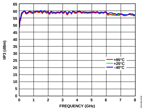
Figure 24. IIP3 vs. Frequency Over Temperature, State = External Bypass A, Path = RFIN to OUT_A or IN_A to RFOUT (Refer to Figure 75 for the Test Circuit)
