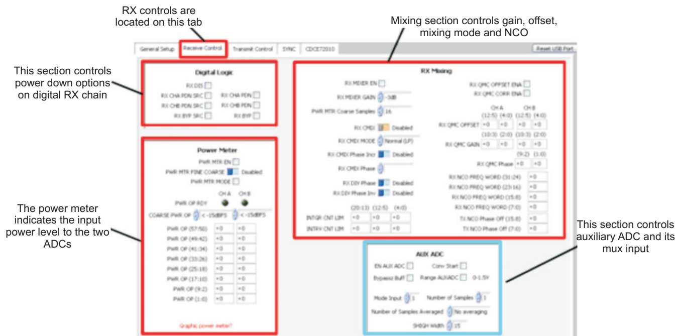
Figure 11. Receive Control Tab in RX Setup
