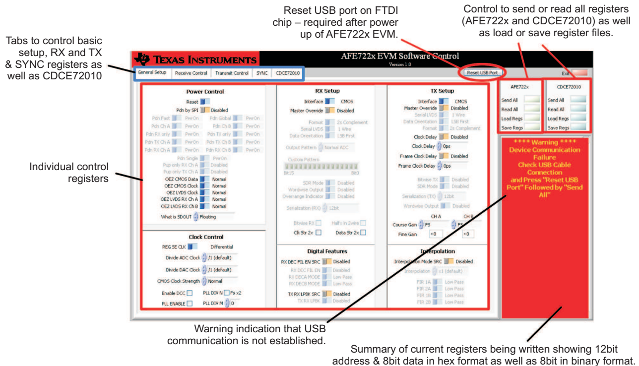
Figure 2. AFE722x EVM Software Control
