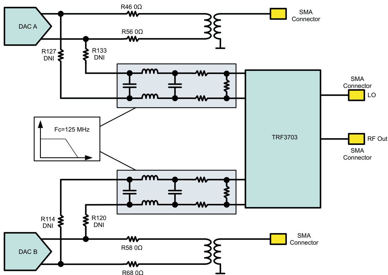
Figure 12. AFE722x Schematic
