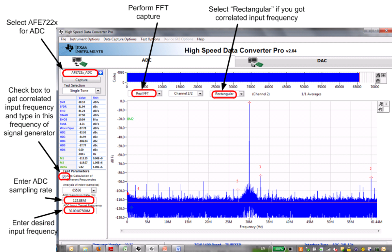
Figure 5. HSDCP Settings
