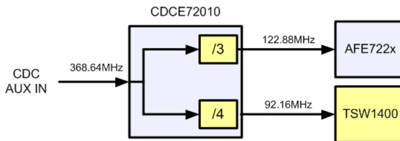
Figure 4. CDCE72010 Configuration
