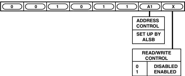
Figure 4. Slave Address
