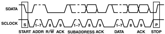
Figure 5. Bus Data Transfer
