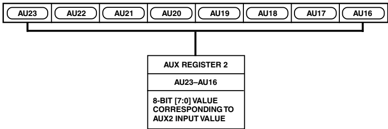
Figure 29. AUX Register 2
