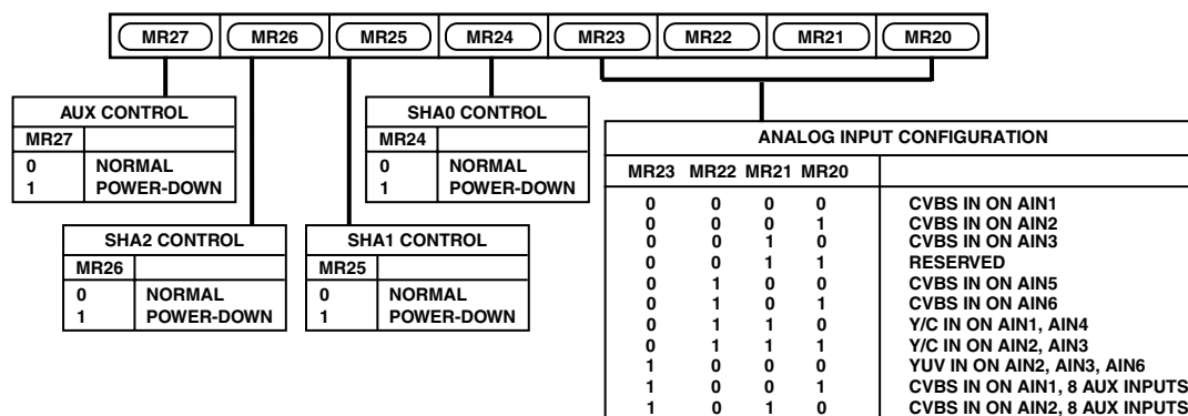
Figure 18. Mode Register 2
