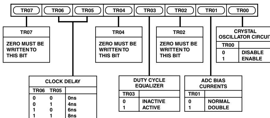
Figure 25. Timing Register 0
