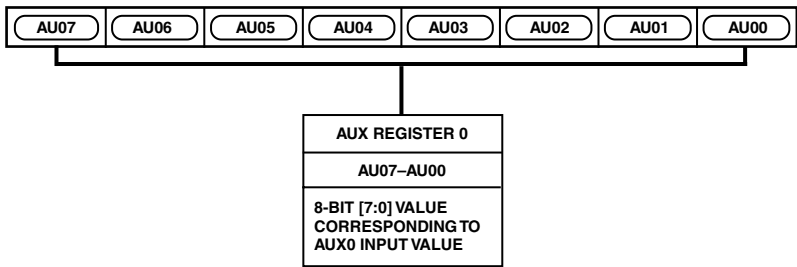
Figure 27. AUX Register 0
