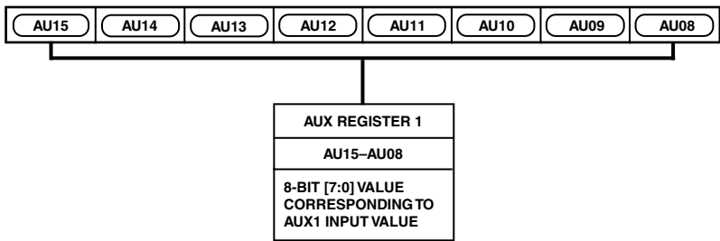
Figure 28. AUX Register 1
