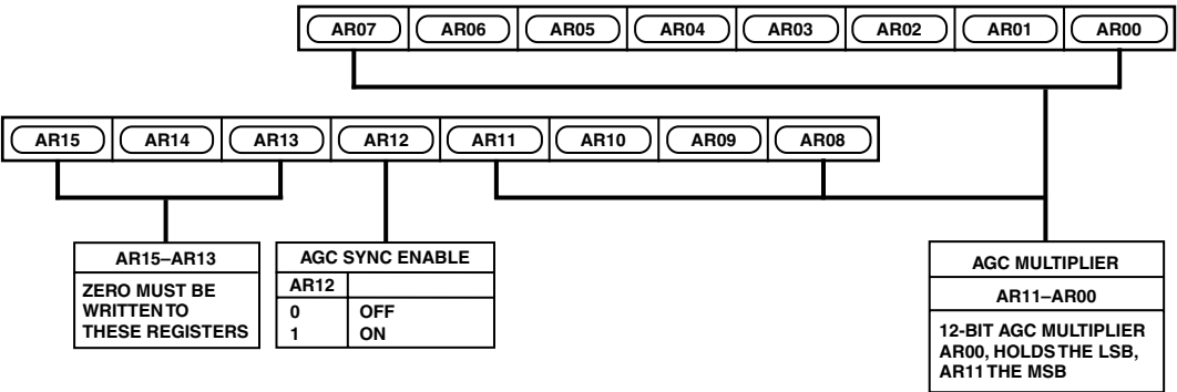
Figure 20. AGC Registers 0-1
