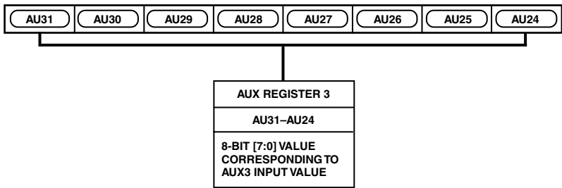
Figure 30. AUX Register 3
