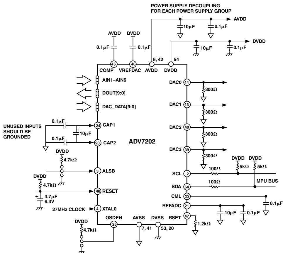
Figure 35. Suggested Schematic
