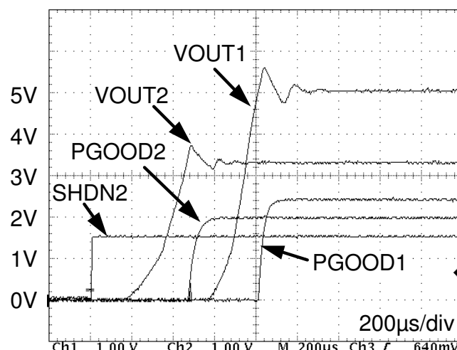
Figure 3. Voltages at start-up with VOUT1 sequenced to VOUT2
