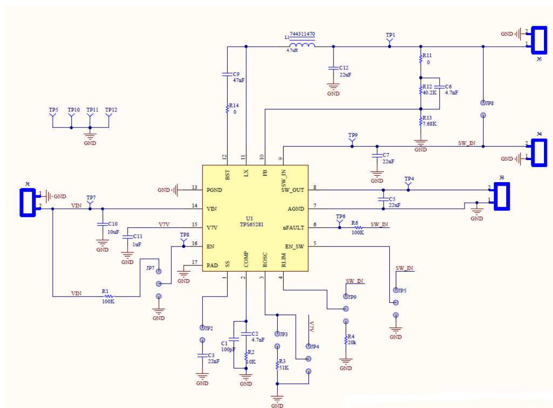
Figure 7. TPS65281EVM Schematic
