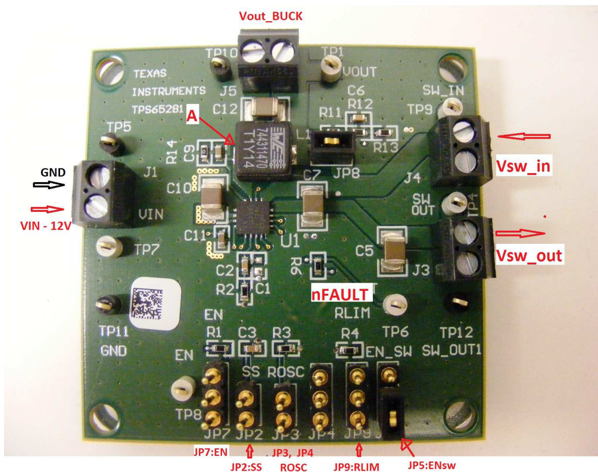
Figure 6. Headers Description and Jumper Placement
