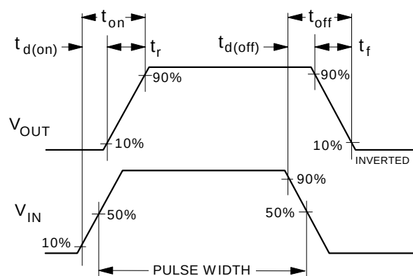
Figure 11. Switching Waveforms.
