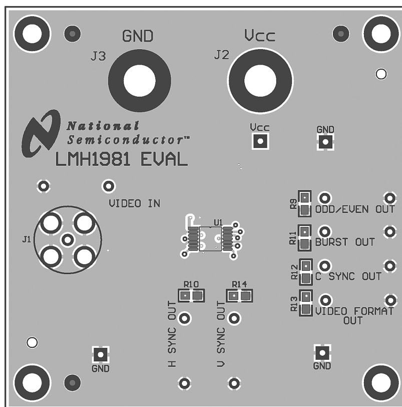
Figure 1. Top Side
