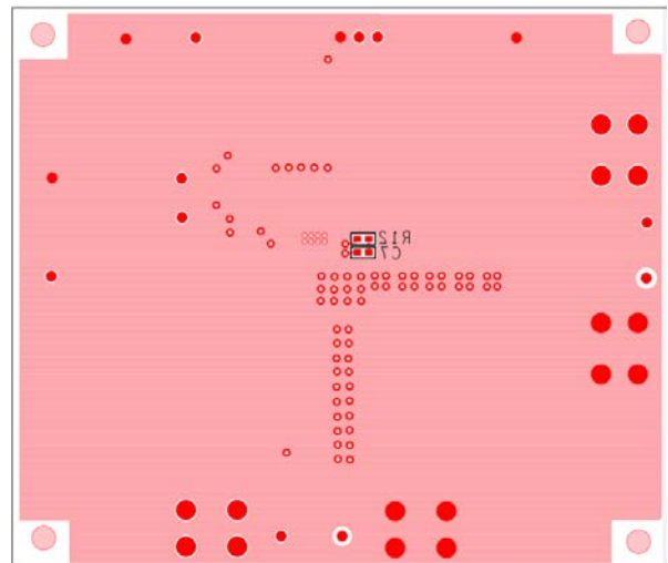
Figure 7. Layer 4, Bottom Side
