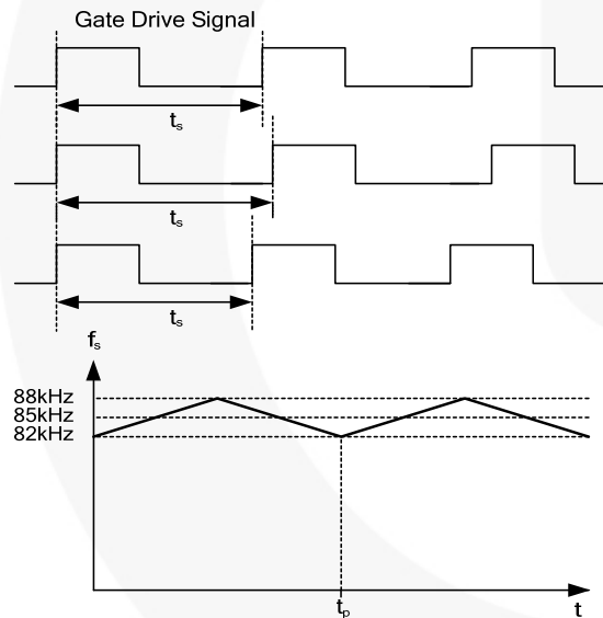
Figure 35. Frequency Hopping
