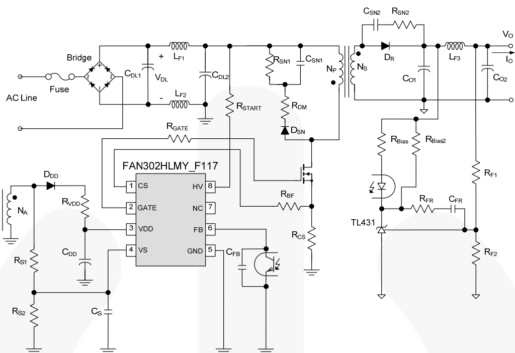
Figure 2. Typical Application
