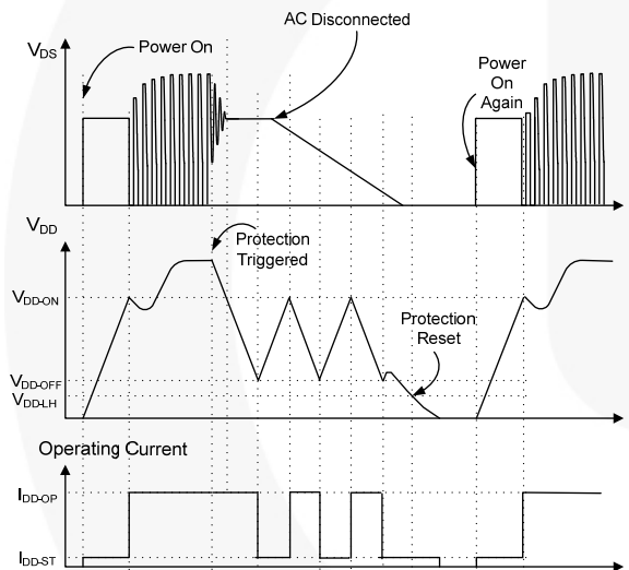
Figure 38. Latch-Mode Operation
