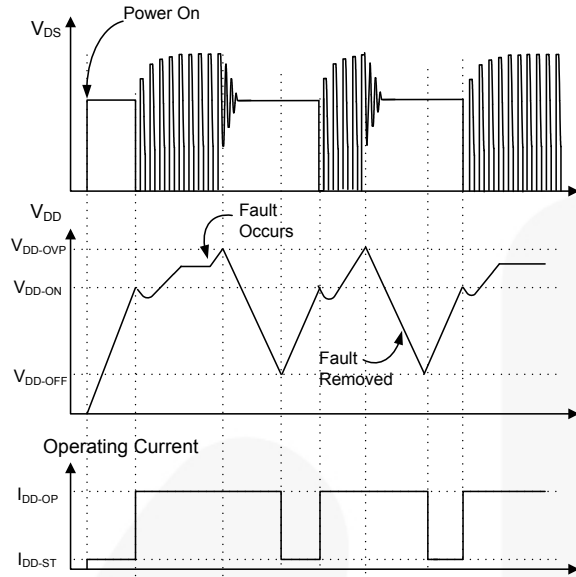
Figure 37. Auto-Restart Mode Operation
