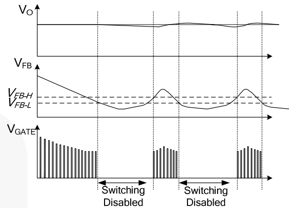
Figure 36. Burst-Mode Operation
