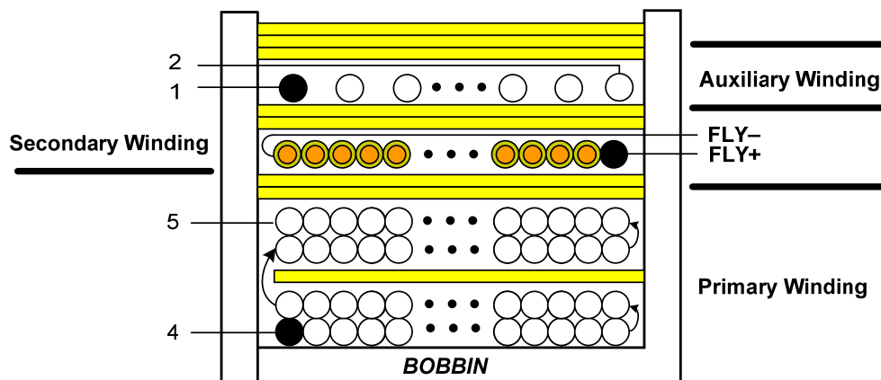
Figure 44. Transformer
