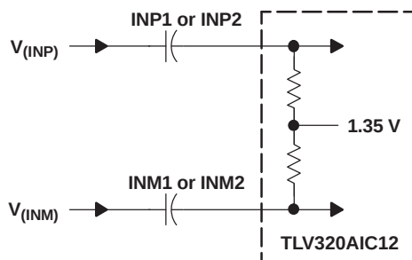
Figure 22. INP and INM Internal Self-Biased Circuit
