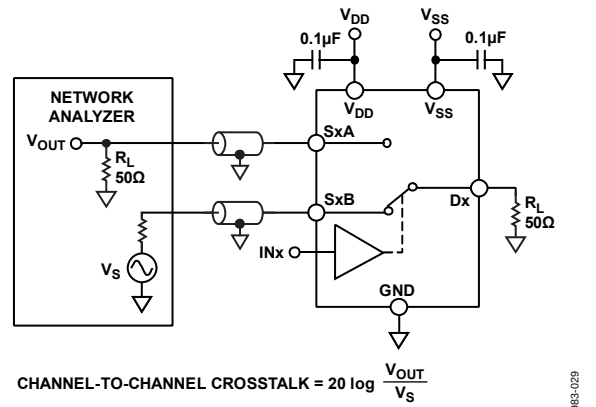
Figure 28. Channel-to-Channel Crosstalk
