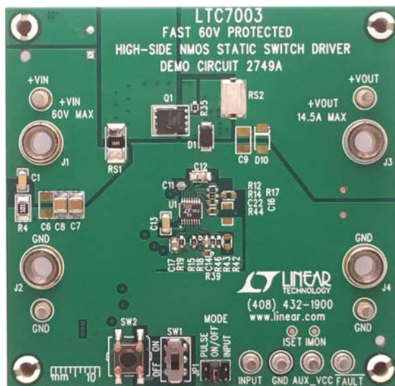
Figure 4. Board Photo
