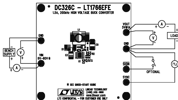
Figure 1. Proper Measurement Equipment Setup
