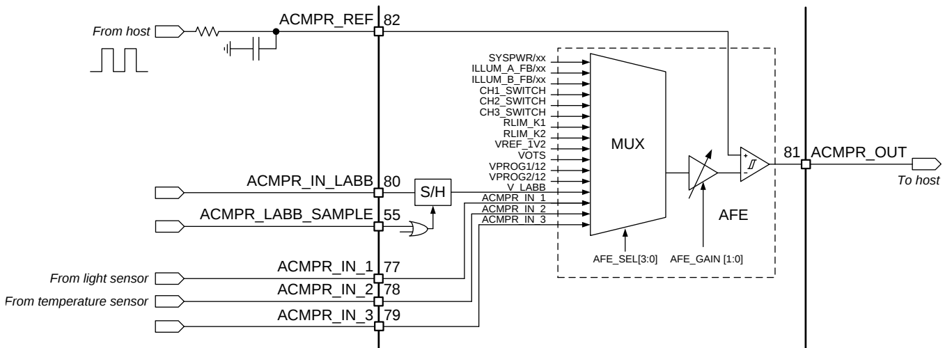
Figure 24. Measurement System
