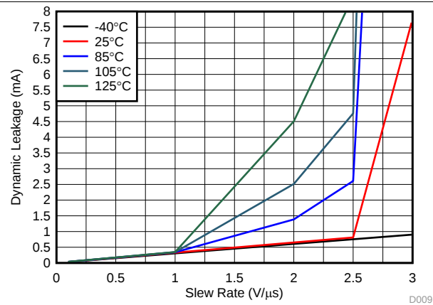
Figure 7. Dynamic Leakage vs Signal Slew Rate Across Temperature
