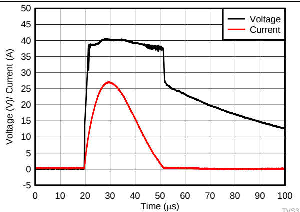
Figure 1. 8/20-μs Surge Response at 27 A
