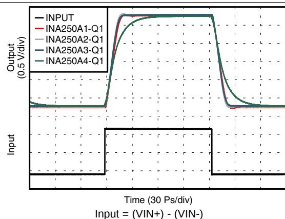
Figure 27. Step Response
