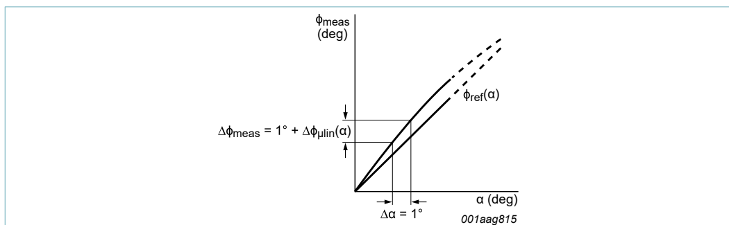
Figure 18. Definition of the microlinearity error
