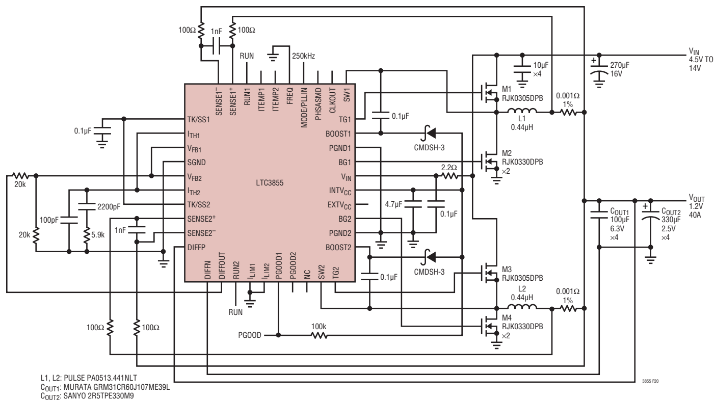
Figure 20. High Efficiency Dual Phase 1.2V, 40A Supply, f_{sw} = 250kHz
