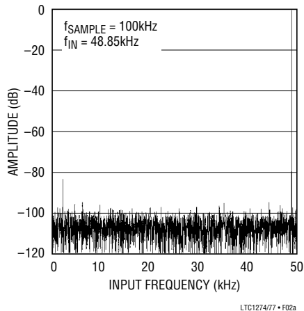
Figure 2a. LTC1274 Nonaveraged, 4096 Point FFT Plot with 50kHz Input Frequency
